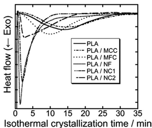
Figure 3. Differential scanning calorimetric thermogram of each sample responsible for the respective isothermal crystallization process at 130°C.
