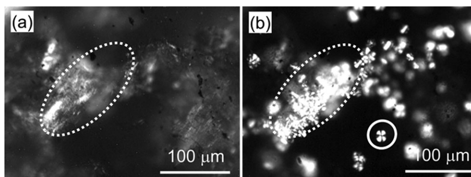
Figure 6. Polarized optical microscopic images showing the relationship between the distribution of NC2 and the microcrystals of PLA in PLA/NC2 (a) before and (b) after isothermal crystallization. The areas surrounded by the dotted line are the same positions in PLA/NC2 before and after the isothermal crystallization. The PLA spherulite is surrounded by a solid line after the crystallization.
